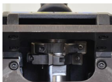
2 rotary milling heads, each holding five 4-sided indexable inserts
