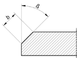
Drawing 1 Bevel dimensions; maximum bevel width depending on the angle
